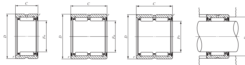
RNA49...U
