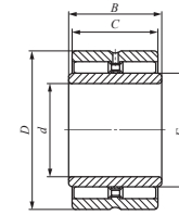
GBRI
