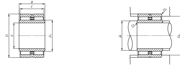
GBRI
