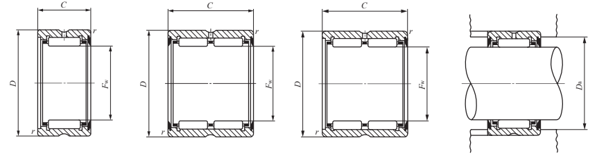
RNA49...U
