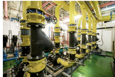
Pumpy
